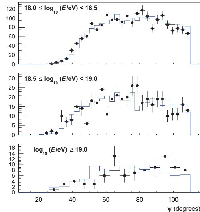
Fig. 6. Data/Monte Carlo comparison for Long Ridge shower inclination angle \psi . Points represent data; the histogram represents Monte Carlo.
