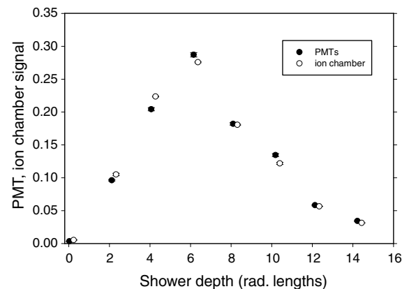
Fig. 10. Comparison of fluorescence and ionization longitudinal profiles. The sums of their points are independently normalized to unity.
