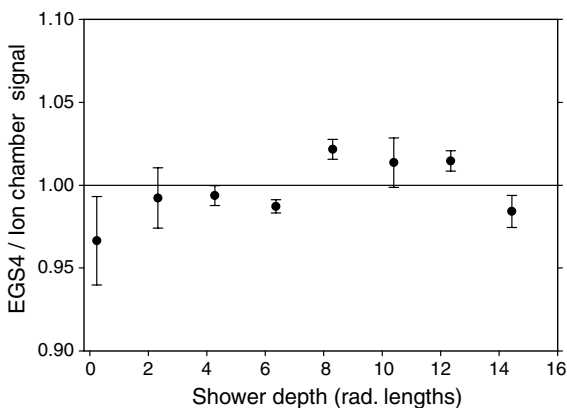
Fig. 5. Ratio of EGS4 simulation to data at each thickness, where the simulation and data depth profiles are both normalized to unity.
