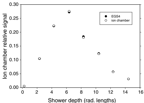
Fig. 4. Ion chamber depth profile and EGS4 simulated depth profiles, both normalized so that the sum of points is unity.
