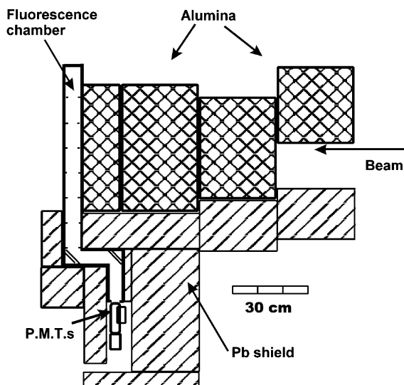
Fig. 2. Plan view of the apparatus. The alumina blocks are shown with the first moved out of the beam (10 radiation length configuration). At left is the air fluorescence detector, its doglegged light pipe and PMTs surrounded by lead shielding. When in place, the scintillation screen and ion chamber would be mounted immediately to the left of the fluorescence volume.
