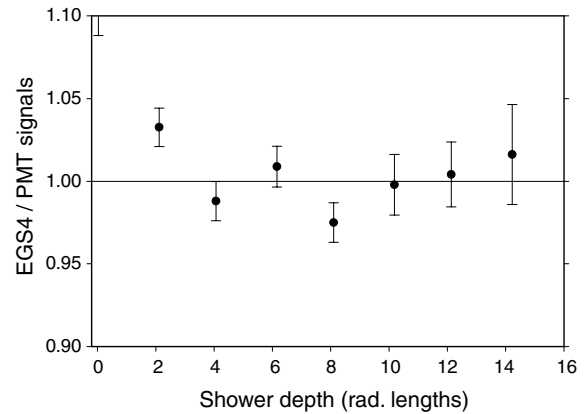
Fig. 9. Ratio of EGS4 results to weighted average of PMT signals vs. shower depth.
