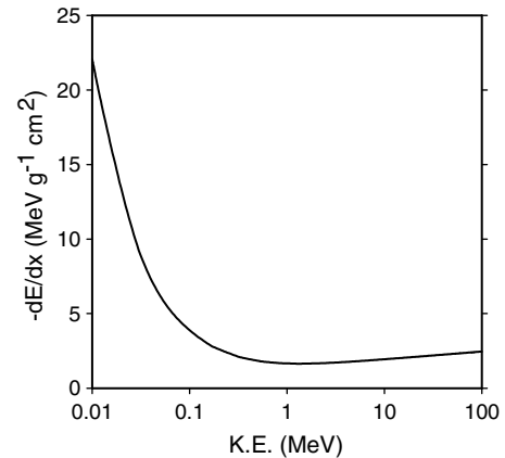
Fig. 1. Energy loss per unit thickness in air vs. particle energy, from the Bethe–Bloch equation.
