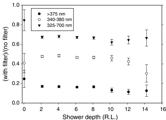
Fig. 11. Comparison between bandpass and wide band optical filters at different shower depths.
