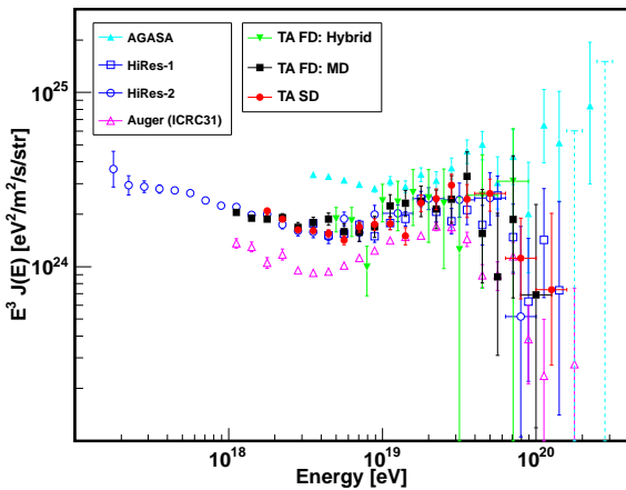
Figure 4: The energy spectra measured by the TA hybrid analysis with other recent experimental data. The dotted line shows the upper limit at 90% C.L.
