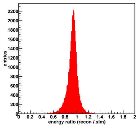
Figure 3: The energy resolution by the hybrid technique. The horizontal axis is the reconstructed energy over true simulation energy. The vertical axis is the number of events. The standard deviation is 8%.
