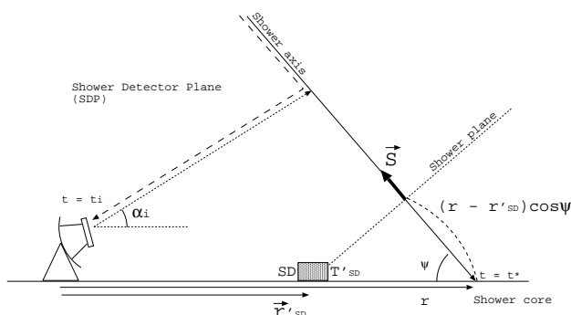
Figure 1: Shower detector plane and the time fit. In this analysis, we assume the shower front as a flat plane.
