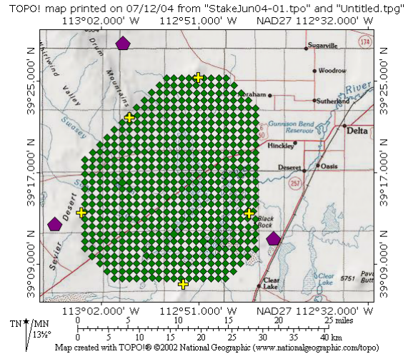
Figure 1. Detector arrangement of the TA SDs ( diamond ) and the FD stations ( pentagon ).
