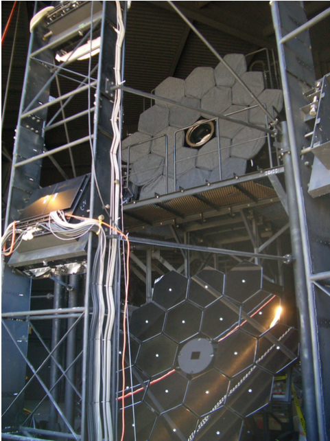
Figure 3. Telescopes and cameras in the first TA FD station. Every segment mirror of the upper mirror has a cover to avoid dust.
