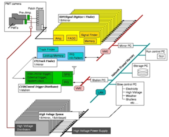
Figure 4. A block diagram of the electronic and the DAQ system in a FD station.
