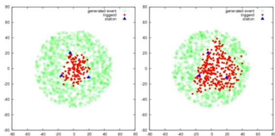
Figure 5. The core locations of the incident cosmic rays ( green open circle ) and the stereo-triggered showers ( red filled circle ) for primary protons of an incident zenith angle of 30^\circ . The primary energies are 10^{19} eV ( left ) and 10^{20} eV ( right ). Each of the blue filled triangles indicates a location of a FD station.
