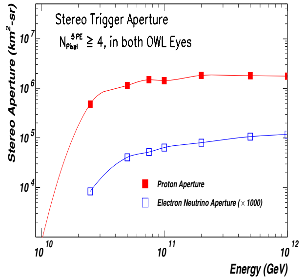
Figure 4. Instantaneous aperture for proton-induced and deep \nu_e -induced giant air-showers as a function of energy.
