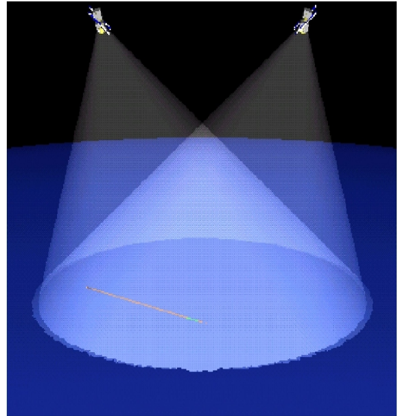
Figure 3. OWL satellites observing the fluorescent track of a giant air shower. The shaded cones show the FOV for each satellite.
