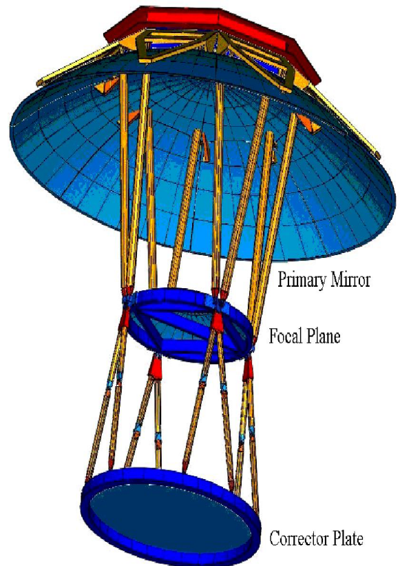
Figure 1. Schematic of the Schmidt optics that form an OWL “eye” in the deployed configuration. The spacecraft bus, light shield, and shutter are not shown.
