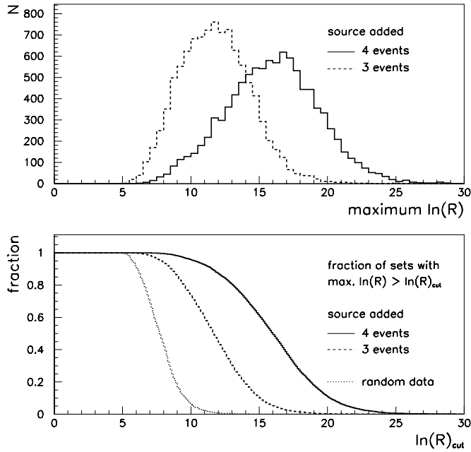
FIG. 5.— Top : Maximum \ln \mathcal{R} for 10^4 simulated random data sets where a four-event source ( solid line ) or a three-event source ( dashed line ) has been added. Bottom : Fraction of simulated data sets with maximum \ln \mathcal{R} > \ln \mathcal{R}_{\text{cut}} as a function of \ln \mathcal{R}_{\text{cut}} for simulated random isotropic data sets with no source added ( dotted line ), a four-event source added ( solid line ), and a three-event source added ( dashed line ).
