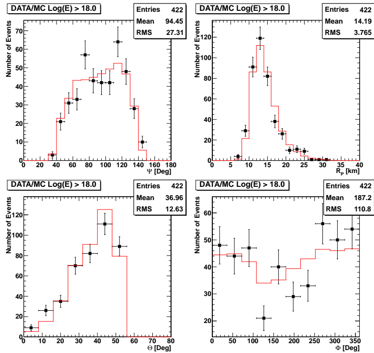
Fig. 4. Comparison of the data and MC distributions in MD events. Each figure is corresponding to the plots in Figure 3.
