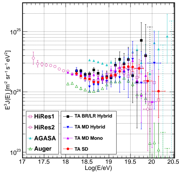
Fig. 5. The energy spectra measured by the TA hybrid analysis with other recent experimental data. The dotted line shows the upper limit at 90% C.L.
