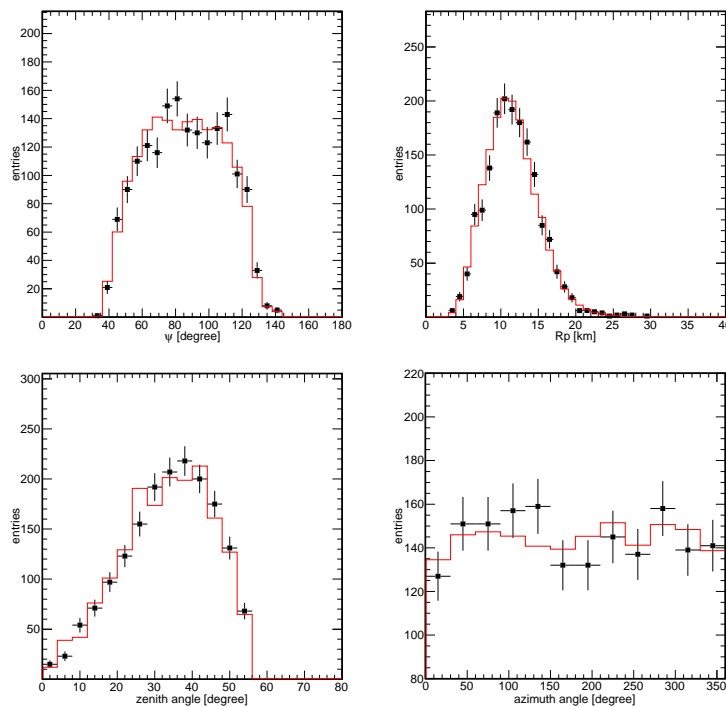
Fig. 3. Comparison of the data and MC distributions in BR and LR events, \psi (left upper), R_p (right upper), zenith angle (left lower) and azimuth angle (right lower). The description of these parameters are in Figure 1.
