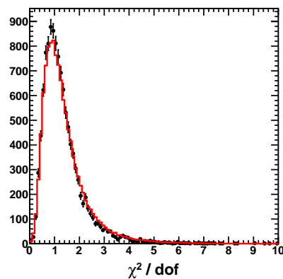
(b) \chi^2/dof of the lateral distribution fit.
