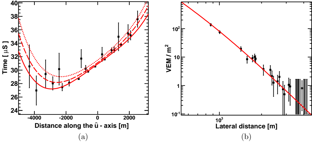
Figure 5.4: Two fits for determining the SD event geometry and S800 . (a): An illustration of the SD time fit. Counter time is plotted versus distance along the \hat{u} -axis (points). Solid line represents the fit expectation time for counters that would lie directly on the \hat{u} -axis, dashed and dotted lines are the fit expectation times for counters that are 1 km and 2 km off the \hat{u} -axis, respectively. (b): Lateral distribution fit to the AGASA function. Counter pulse height is plotted versus the perpendicular (lateral) distance from the shower axis. Solid line represents the fit curve. Error bars with no points represent the silent counters (working counters which did not register any signal).
