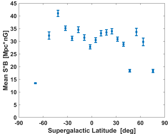
Figure 16. Mean B \times S inside equal solid angle SGB bins not counting wedges with positive correlations. These values are independent of the ranked correlation pre-trial significances, which were maximized to choose the wedge parameters. The mean within |SGB| \leq 40^\circ is \langle B \times S \rangle = 32 nG*Mpc. If proton is the assumed composition, then the average coherent field component, perpendicular to the FOV, in the vicinity of the supergalactic plane assuming a distance of 3.7 Mpc is 8.6 nG.
