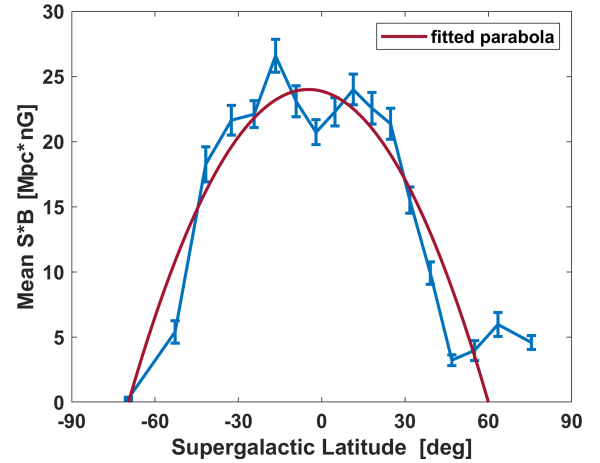
Figure 15. Mean B \times S inside equal solid angle SGB bins setting B \times S = 0 for wedges with positive correlations. The fitted parabola also demonstrates the correlation between apparent magnetic deflection multiplets with the supergalactic plane. These values are independent of the ranked correlation pre-trial significances, which were maximized to choose the wedge parameters. The mean within |SGB| \leq 40^\circ is \langle B \times S \rangle = 21 nG*Mpc. If proton is the assumed composition, then the average coherent field component, perpendicular to the FOV, in the vicinity of the supergalactic plane assuming a distance of 3.7 Mpc is 5.6 nG.
