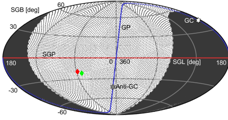
Figure 2. A supergalactic Hammer-Aitoff projection of the equal distance oversampling grid. This is a grid of 6553 points with a mean spacing of 2.1 \pm 0.1^\circ . The grid boundary is defined by the equatorial edge of the field of view at Dec. = -16^\circ . The red diamond is the location of the Hotspot (Abbasi et al. (2014)), and the green diamond is the location of the energy spectrum anisotropy (Abbasi et al. (2018a)). The red line is the supergalactic plane (SGP) and the blue line is the galactic plane (GP).
