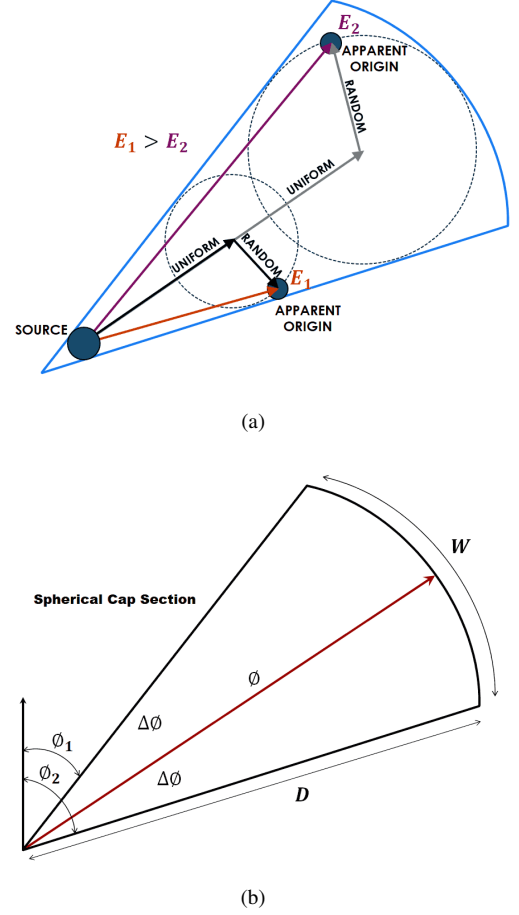
Figure 1. Pictograph of UHECR Drift-diffusion deflection “wedge” bins (spherical cap sections) displayed on a flat space. (a) Two different energy events having traveled through coherent and random magnetic fields. The purple vector represents the low energy event spherical arc, and the red vector is a higher energy event. Coherent and random magnetic field components describe the average perpendicular to the field-of-view (FOV) sphere. Dashed circles represent possible random field RMS deflections. (b) A spherical cap section (wedge) is a simple shape that best encompasses the likeliest positions. Pointing direction is the spherical arc \phi , \Delta\phi is the wedge width, and D is the maximum angular distance (spherical cap radius).
