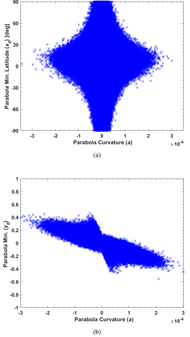
Figure 6. The behavior of the three mean \tau parabola fit parameters (Figure 5(b)) with respect to each other in random isotropic MC simulations. (a) The parabola fit curvature, a , versus minimum supergalactic latitude (SGB), x_0 , shows that a high curvature tends to a minimum near the supergalactic plane. (b) The parabola fit curvature, a , versus the fit minimum value, y_0 , shows that a high curvature tends to a higher magnitude negative mean \tau .
