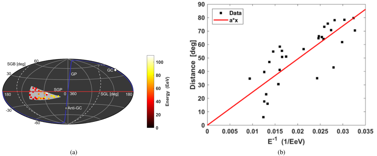
Figure 3. (a) A supergalactic Hammer-Aitoff projection of the seven years data spherical cap section, or “wedge”, with the maximum significance at 18.3^\circ SGB, -12.9^\circ SGL. The correlation strength is \tau = -0.675 , and with 29 data events has a pre-trial one-sided significance of 5.5\sigma . The energy threshold is E_i \geq 30 EeV, wedge width W_i = 30^\circ , distance D_i = 80^\circ , and direction \phi_i = 90^\circ . (b) A scatter plot of 1/E_j versus distance \delta_{ij} for events in the wedge. A linear fit (by Equation 1a with Z=1 ) results in an estimate of B \times S = 49 nG*Mpc. If the source is assumed to be the same distance as M82 (3.7 Mpc) with a pure proton emission, then the coherent magnetic field required to cause this deflection would be B = 13 nG.
