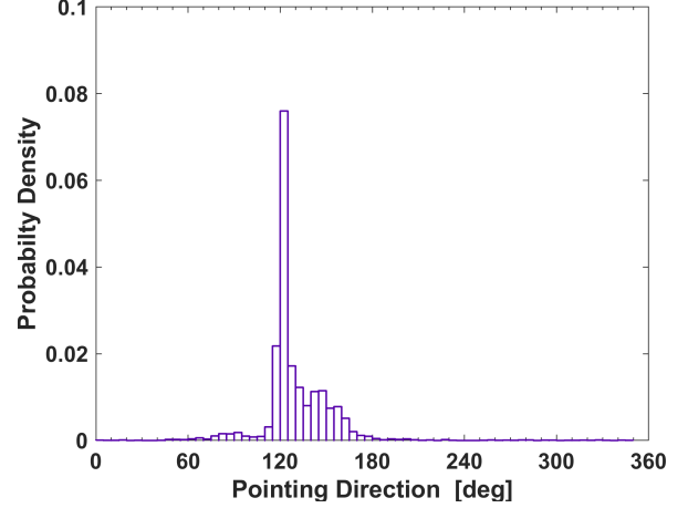
Figure 14. Distribution of pointing direction of wedges found in randomized data with the most significant wedge embedded.
