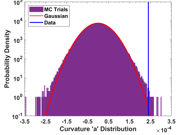
Figure 9. The distribution of the curvature parameter a of the mean \tau parabola chosen as the supergalactic structure of multiplets test statistic for 1,000,000 isotropic MC sets. The purple bars are the MC probability distribution function (PDF). The red line is a Gaussian distribution fit to the MC distribution. The curvature for the data is a=2.45\times 10^{-4} shown as a blue vertical line. There are 14 MC with a larger curvature than data, which gives a significance of 4.2\sigma .
