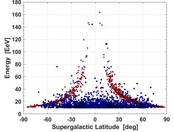
Figure 4. Toy-model supergalactic magnetic sheet simulation. Blue circles are the F = 65.7\% isotropic fraction of MC events. Red squares are the anisotropic MC events magnetically diffused away from the supergalactic plane with B \times S=18.47 nG*Mpc. Overall, event positions are isotropic, and the energy spectrum is created according to the published HiRes/TA result.
