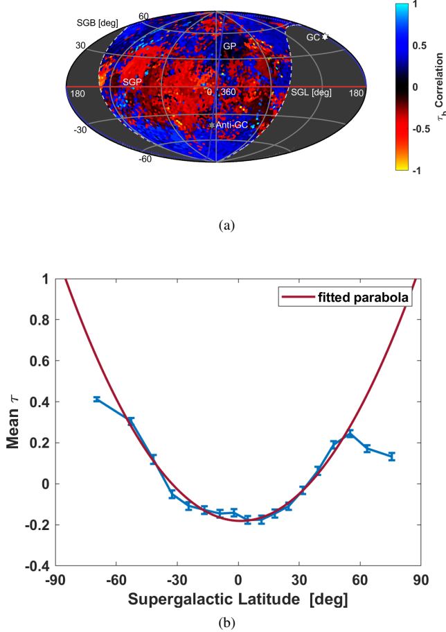
Figure 8. Ten years of data result. (a) Projection of the correlation strength \tau for all grid points. Negative correlations expected for magnetic deflections are apparent around the supergalactic plane. (b) Mean \tau inside equal solid angle bins of supergalactic latitude (SGB). The correlation curvature is a=(1.60\pm 0.09)\times 10^{-4} .
