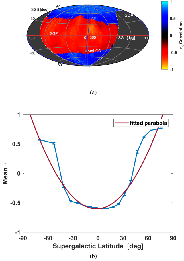
Figure 5. A supergalactic magnetic sheet simulation. (a) Projection of the correlation strength \tau for all grid points. Solid curves indicate the galactic plane (GP) in blue and supergalactic plane (SGP) in red. (b) Mean \tau inside equal solid angle bins of supergalactic latitude (SGB). The parabolic fit ( y = a(x - x_0)^2 + y_0 ) shows the curvature parameter, a , chosen as the test statistic. a = 2.5 \times 10^{-4} .
