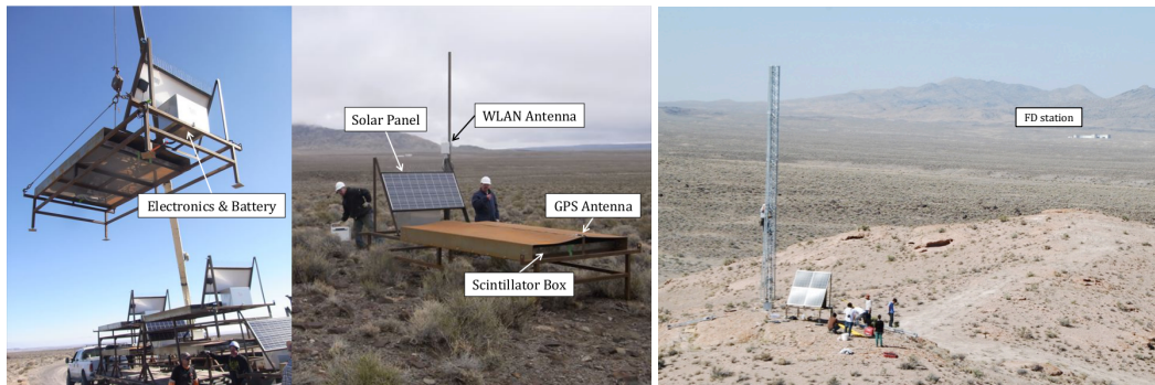
Figure 2: ( left ) A deployed SD in the field. The electronics box and scintillator box are on the iron frame. An electronics unit is installed under the solar panel, and the scintillator box is mounted on the platform under the roof. ( right ) The Middle Drum communication tower for the TALE SD array. There are four solar panels for the power supply, and the stand for the panels contains batteries, host PC and network instruments. The Middle Drum FD station is visible in the distance.
