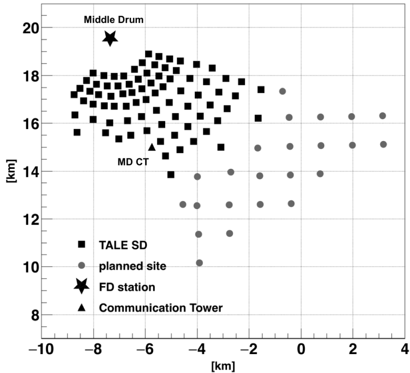
Figure 1: The layout of the TALE in Utah, USA. Squares denote 80 SDs and circles are the planned locations of SDs for the connecting region between TA and TALE. The array controlled with a host PC at the communication tower denoted by a triangle and labeled "MD CT". The star symbol denote the Middle Drum station of the TA FDs and the TALE FDs.
