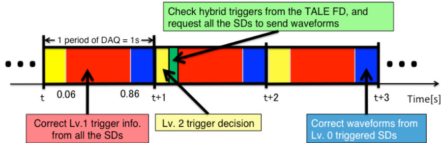
Figure 4: This is a time chart of the DAQ cycle of the TALE SD array. For each period the start-point is synchronized with the GPS PPS signal. The single DAQ cycle to record an air shower event data continues in the following steps. (1, Red) The host PC requests/receives the most recent Level-1 trigger information including a Level-1 trigger time table. (2, Yellow in the next period) Event trigger, called Level-2 trigger, decision. (3, Green) Check hybrid trigger signals. With the Level-2 or the hybrid trigger trigger the host PC requests each SD to transfer waveform data. (4, Blue, in the following periods) The host PC corrects waveforms.
