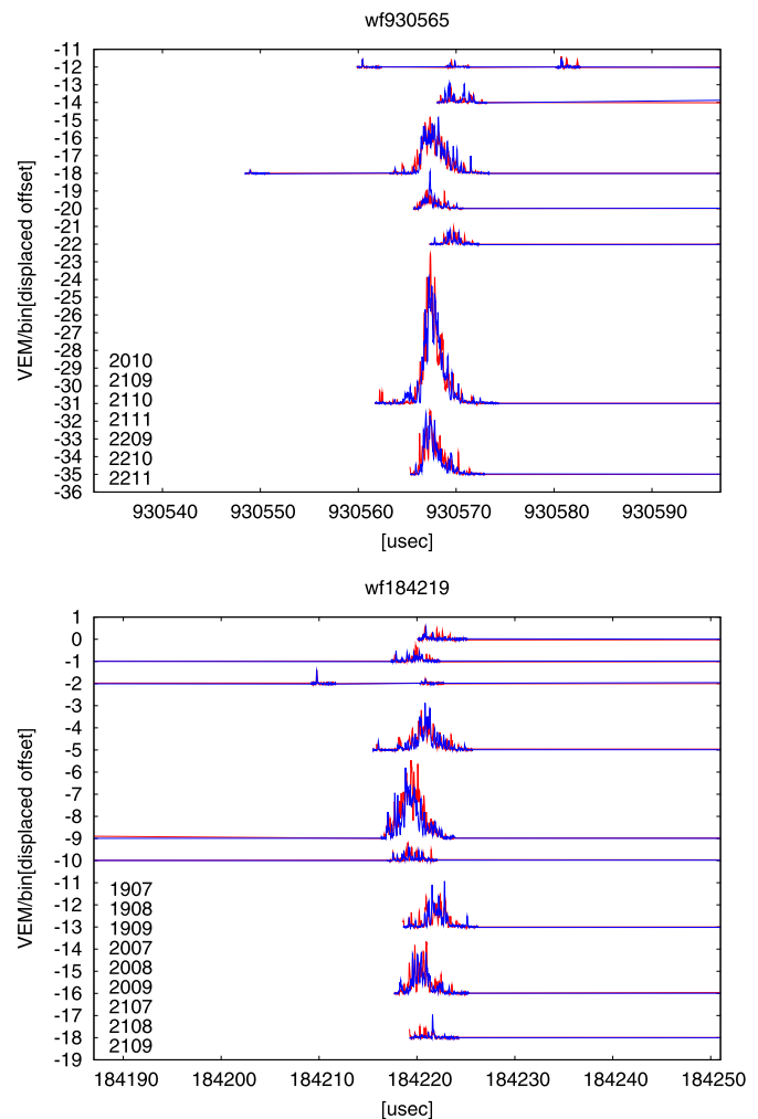
Fig. 10. Gaussian like waveforms from SDs in the vicinity of the shower core. Red and blue correspond to two PMT channels for two layers of scintillator. Each horizontal level corresponds to the pedestal of individual SD. Vertical value has been shifted to avoid superposition of waveforms from different SDs. (For interpretation of the references to color in this figure legend, the reader is referred to the web version of this article.)
