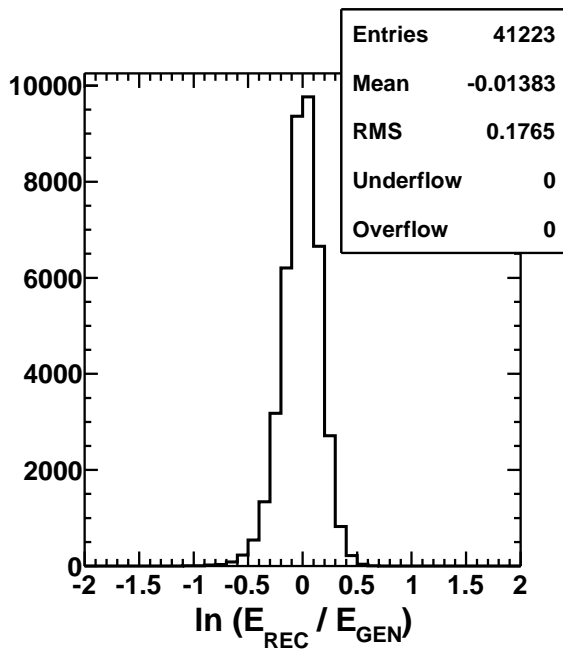
Fig. 9: Energy resolution of the TA SD evaluated by the Monte-Carlo. The histogram shows the distribution of the natural logarithm of the reconstructed ( E_{\text{REC}} ) energy divided by the true energy ( E_{\text{GEN}} ).
