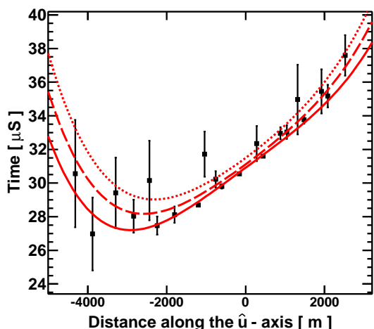
Fig. 2: TA SD time fit. Counter time is plotted versus the distance from the shower core along the \hat{u} direction, which is the projection of the shower axis on the ground. Points with error bars are counter times, solid curve is the time expected by the fit for the counters lying on the \hat{u} axis, dashed and dotted lines are the fit expectation times for the counters that are correspondingly 1.5 and 2.0 km off the \hat{u} axis.
