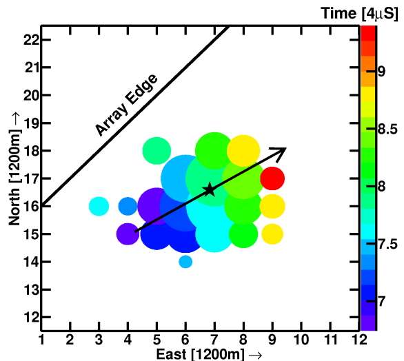
Fig. 1: A typical high energy event seen by the TA SD. Each circle represents a counter, positioned at the center of the circle, the area of the circle is logarithmically proportional to the counter pulse height, and the counter time is denoted by the color. The arrow represents the projection of the shower axis onto the ground, which we label by \hat{u} , and it is bisected by the perpendicular line at the location of the shower core.
