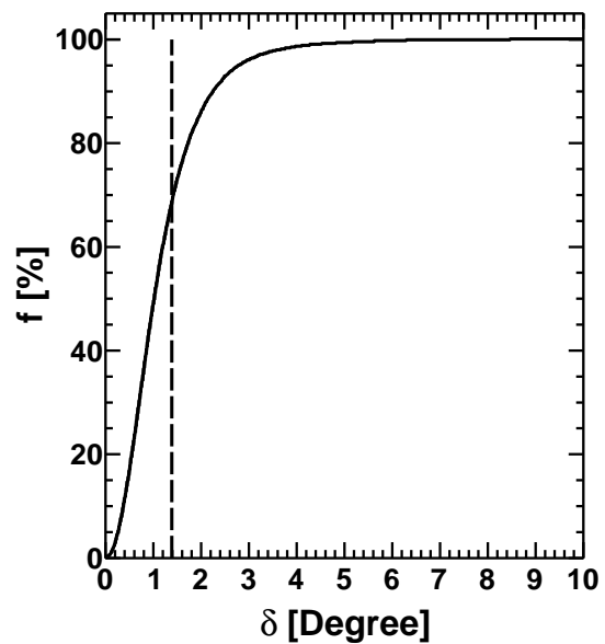
Fig. 8: Angular resolution of the TA SD evaluated by Monte-Carlo. Fraction of events ( f ) reconstructing within a certain opening angle ( \delta ) of the true event direction is plotted versus the opening angle. 68% of events reconstruct within 1.4^\circ of the true event direction.
