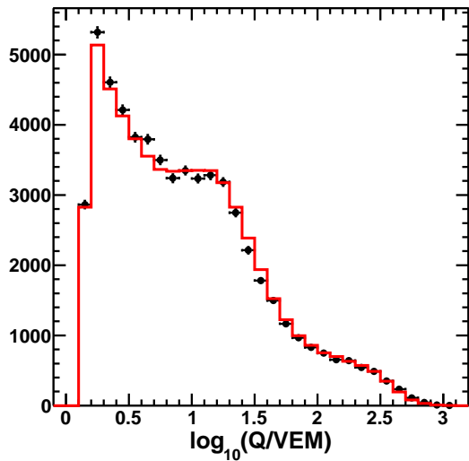
Fig. 5: Data and MC comparison of counter pulse height. The points with error bars represent the data histogram and the solid line represents the MC.
