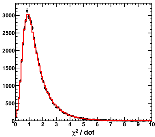
Fig. 6: TA SD data and MC comparison of the lateral distribution fit \chi^2 per degree of freedom.
