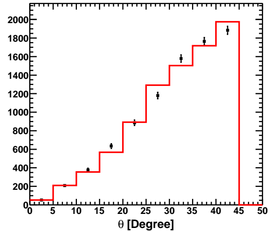
Fig. 7: Data and MC comparison of the event zenith angle.
