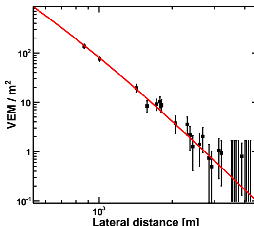
Fig. 3: Lateral distribution profile fit to the AGASA LDF. Vertical axis is the signal density and horizontal axis is the lateral distance from the shower core.
