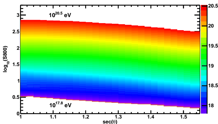
Fig. 4: Energy as a function of reconstructed S800 and \sec(\theta) made from the CORSIKA MC. Z-axis described by color represents the true (MC generated) values of energy.
