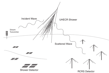
Fig. 1: The geometry for a radar echo technique.
