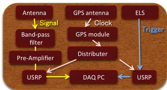
Fig. 4: The schematic view of the DAQ system.
