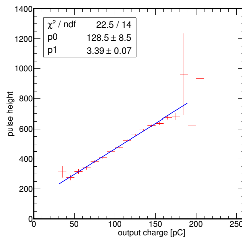
Fig. 7: The beam charge dependence of the observed signals. The horizontal axis is the output beam charge measured at the ELS. The vertical axis is the pulse height of the observed signal at the receiver.
