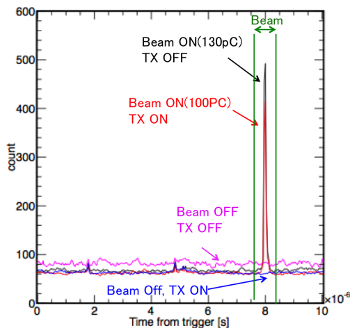
Fig. 6: The observed signal in the short pulse beam experiment, which is same format of Fig. 5. In this experiment, the total gain of the amplifiers is 30dB. Four signals obtained from the difference configuration are shown.
