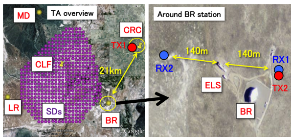
Fig. 2: The overview of the TA site. The positions of transmitters (TX), receivers (RX) and ELS are shown.
