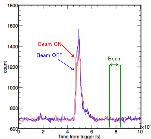
Fig. 5: The observed signal in the long pulse beam experiment with averaged about \sim 1000 events. In this experiment, the total gain of the amplifiers is 50dB. The horizontal axis is the time from the ELS trigger. The vertical axis is the ADC count. The red line is observed signal with shooting the electron beam, and the blue line is the signal without beam.
