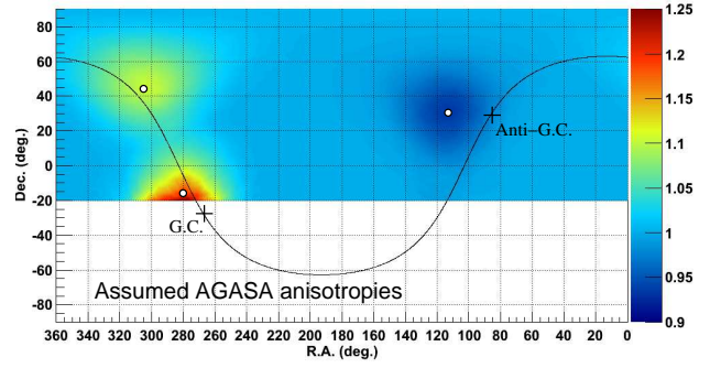
Fig. 2: Assumed AGASA anisotropy formed by the 2D Gaussian shape with the \sigma_s = 13^\circ . The color contour shows the relative intensities which are averaged over 20^\circ radius circle at each coordinate. The open circles show the center positions of assumed the AGASA anisotropies [1]. The cross marks indicate the Galactic center (G.C.) and the Anti-Galactic center (Anti-G.C.), while the solid curve indicates the Galactic plane.
