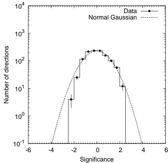
Fig. 4: Histogram shows significance distribution of samples on the grid 3^\circ spacing in the map as shown in Fig. 3(b). The dashed curve is the expected normal Gaussian distributions.
