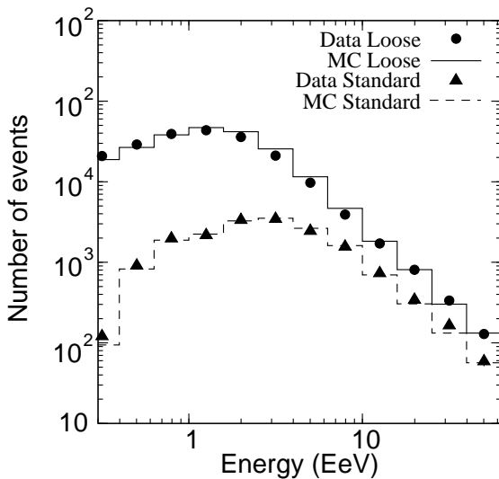
Fig. 1: Reconstructed energy spectra. Closed circles and triangles show energy spectra of the experimental data after the loose and standard cuts, respectively. Solid and dashed histograms show energy spectra by the MC simulation after the loose and standard cuts, respectively.
