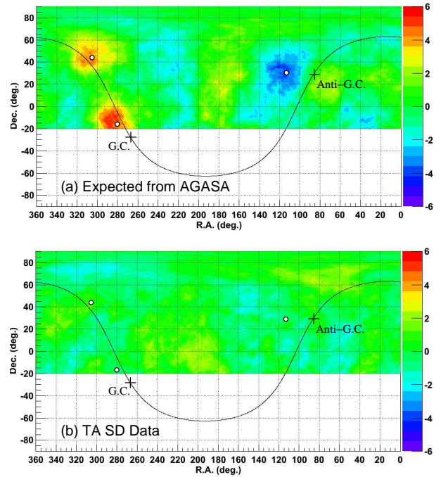
Fig. 3: (a): Expected significance map with the TA SD using the MC sample events assuming the AGASA anisotropies as shown in Fig.2. The number of analyzed events is the same statistics of the air shower events observed by the TA SD. (b): Actual significance map of the anisotropy observed by the TA SD in the energy range between 10^{18.0} eV and 10^{18.4} eV. The events in maps are summed over 20^\circ radius circles centered at 1^\circ \times 1^\circ grids on the equatorial coordinate. The open circles show the center positions of assumed anisotropies. The cross marks indicate the Galactic center (G.C.) and the Anti-Galactic center (Anti-G.C.), while the solid curve indicates the Galactic plane.
