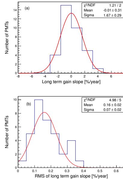
Fig. 5: Long-term behavior of (a) PMT gain slopes and (b) their systematic deviations for the 35 selected PMTs measured by the YAP.
