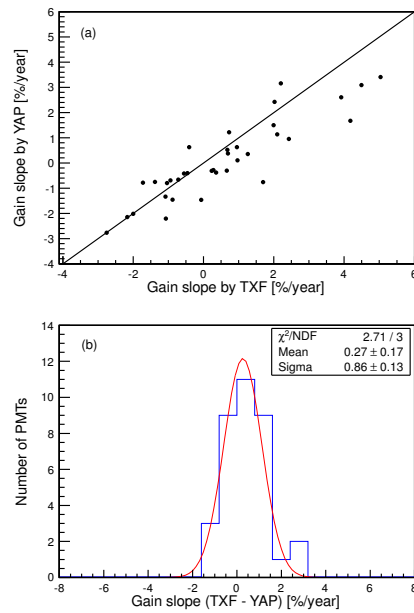
Fig. 8: (a) scatter plot of long-term gain slopes and (b) the difference of long-term gain slopes measured by the YAP and TXF calibrations.
