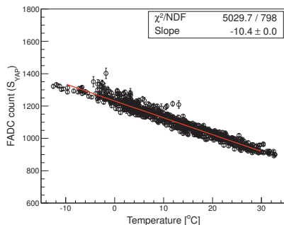
Fig. 3: Behavior of the YAP signals as a function of ambient temperature of the camera in the #LR00 telescope at 2008.
