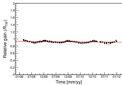
Fig. 6: History of relative gain ( R_{TXF} ) for the standard PMT in the #LR00 telescope. Seasonal variation of R_{TXF} in the figure is due to temperature coefficient of each PMT.
