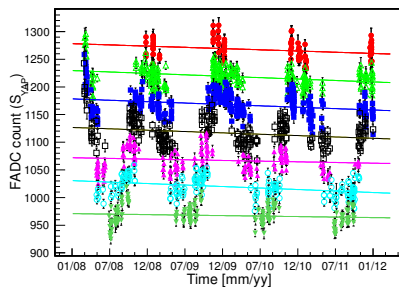
Fig. 2: Seasonal variation of YAP signal for the standard PMT in the #LR00 telescope. Color-markers with fitted line is subsets of temperature range 5^\circ\text{C} step from -5^\circ\text{C} (top) to +25^\circ\text{C} (bottom)
