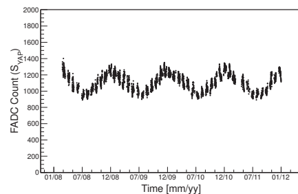
Fig. 1: History of S_{\text{YAP}} for the standard PMT in the #LR00 telescope over 4 years.
