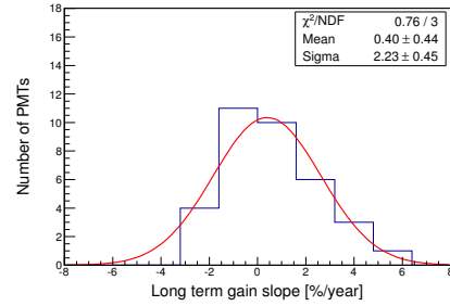
Fig. 7: Distribution of long-term gain slopes measured by the TXF.
