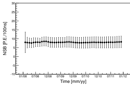
Fig. 9: History of night sky background level over 4 years observed at the standard PMT in the #LR00 telescope. Each data point and its error denote the mean and standard deviation obtained from a Gaussian fit with one month data, respectively.
